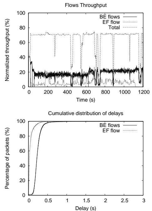
Fig. 4. Scenario 1: Throughput and cumulative distribution of delays in the network without QoS control
