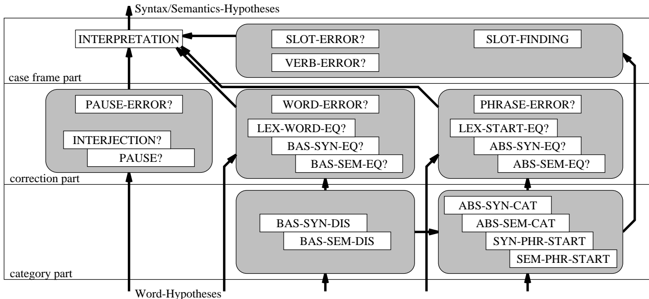
Figure 2: SCREEN: some modules of the category, correction, and case frame parts
