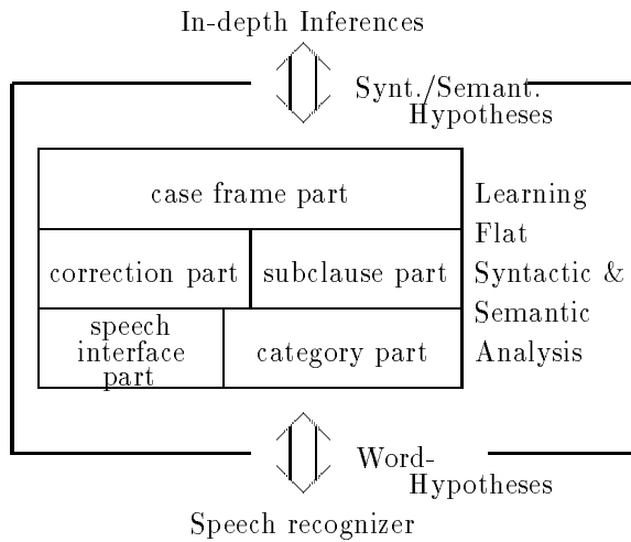
Figure 1: Overview of SCREEN
